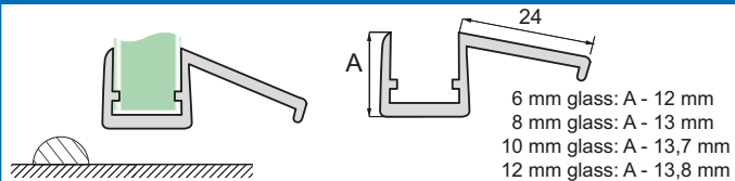
Glass to Floor S-5720
