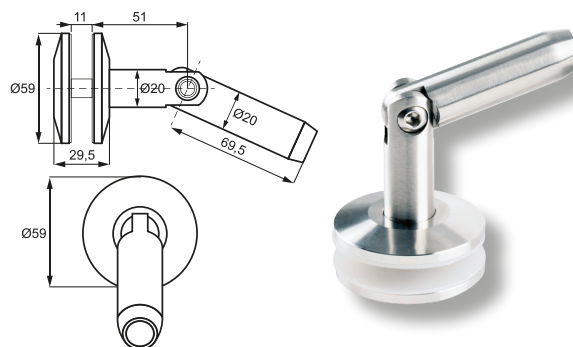
Rod connector 1000 mm # 22.10.503
