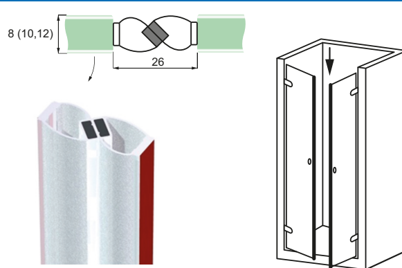
Glass to Glass ADH07 - W/magnet - 180° - Frosted
