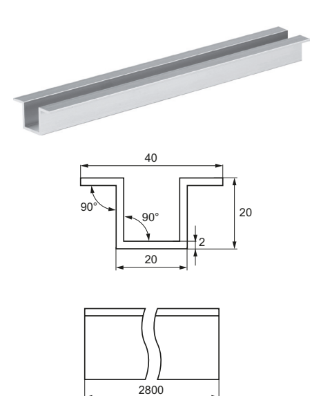
Aluminium bottom profile - 2800 mm - brushed Item No.: # 28.25.221
