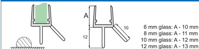
Glass to Floor S-5722
