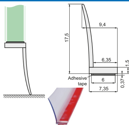
Glass to Floor ADH02 - Clear
