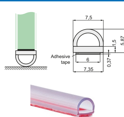
Glass to Floor ADH03 - Clear
