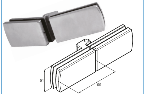
Bottom folding hinge w/guide pin Item No.: # 28.29.055
