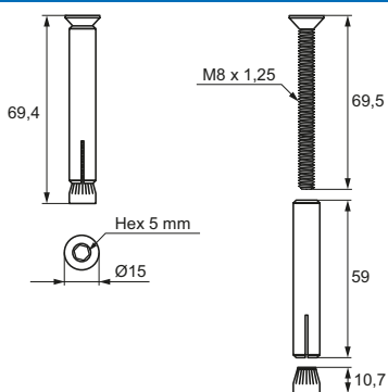
Expansion Bolt SS-316, M8 x 1,25 x 70 mm # 22.10.502-9
