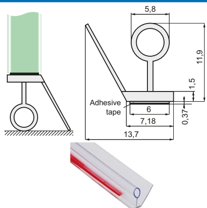
Glass to Floor ADH01 - Clear
