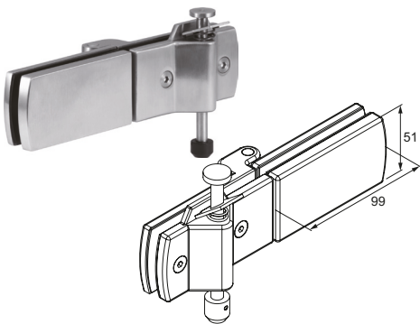
Bottom start pivot hinge Item No.: # 28.29.056
