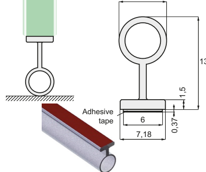
Glass to Floor ADH05 - Frosted
