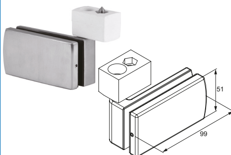
Glass Door Lock Item No.: # 14.60.642
