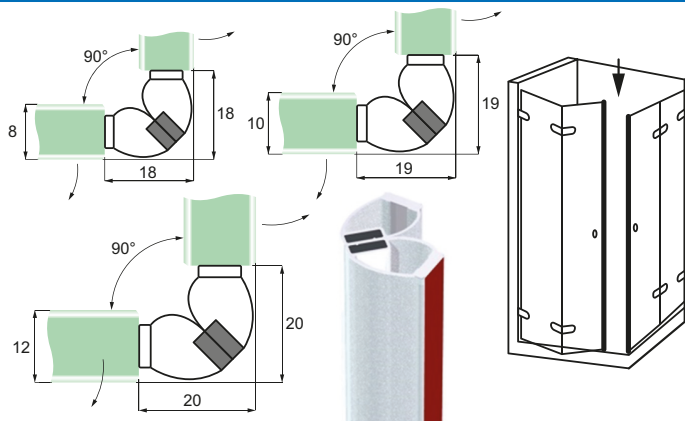
Glass to Glass ADH06 - W/magnet - 90° - Frosted
