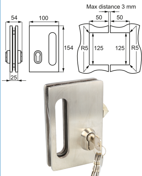
Glass Door Lock Item No.: # 14.60.642
