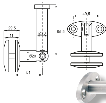
Wall/rod corner connector # 22.10.502
