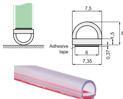
Glass to Floor ADH04 - Frosted
