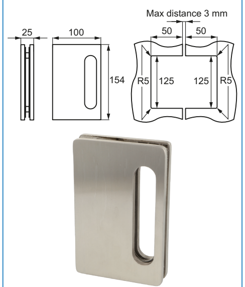
Striker for Glass door lock 14.60.642 Item No.: # 14.60.643
