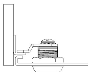
Installation diagram
